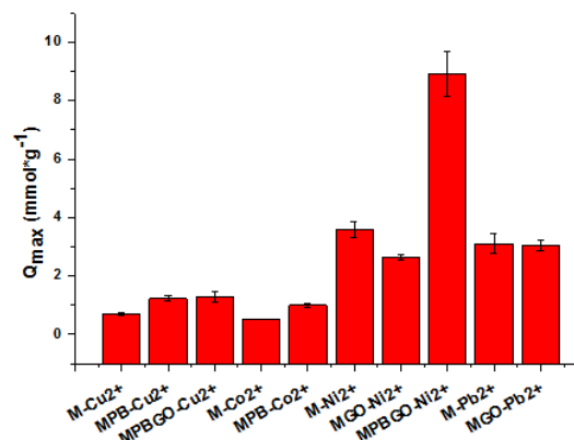
Figure 1. Q_{\max} values for nano-magnetic sorbents.
