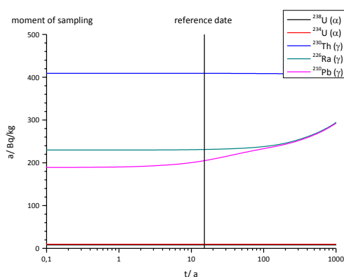
Figure 1. Evolution of the specific activities a with time t of members of the 238 U decay chain in sediment IAEA-410.
