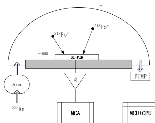
Figure 1. Structure of the radon measurement equipment
