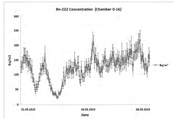
Figure 1. Radon concentration within the Liquid Treatment Centre
