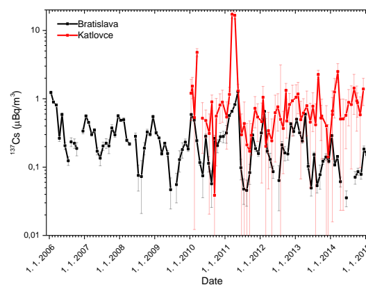
Figure 1. Concentrations of ^{137}\text{Cs} in Bratislava and Katlovce.
