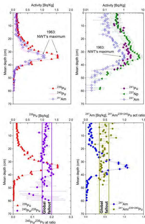
Figure 2. Vertical profiles of some of the investigated radionuclides and isotope ratios.
