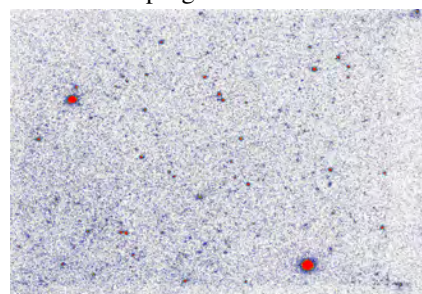
Figure 1. Autoradiography image of filter collected between 27-28 April 1986
