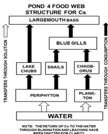
Figure 1. Pond 4 Modeled 133 Cs Biotic Pathways
