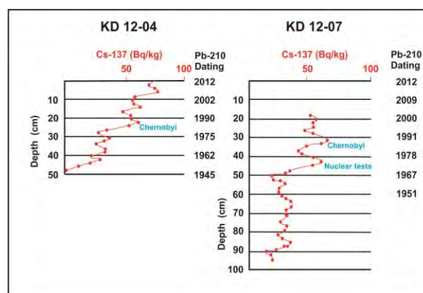
Figure 2. Distribution of 137 Cs activity and 210 Pb dating in cores.
