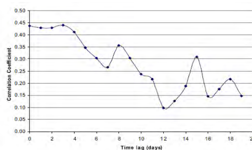
Figure 1. Day lag plot for the region of Thessaloniki.
