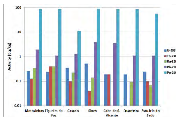
Figure 2. Concentrations of natural radionuclides in mussels (year 2015).
