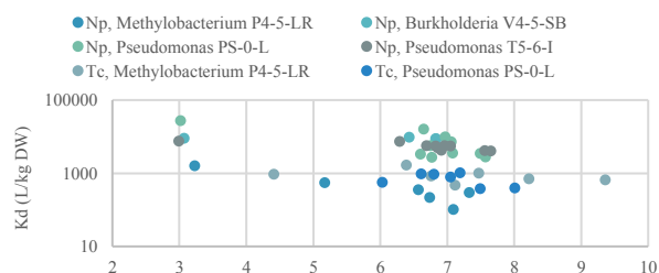
Figure 2. Np and Tc uptake as a function of pH
