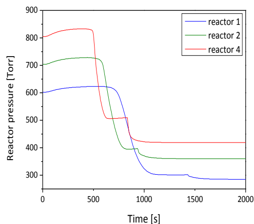
Figure 1. History of preparation of \text{TiH}_2 from hydrogen gas and titanium powder.
