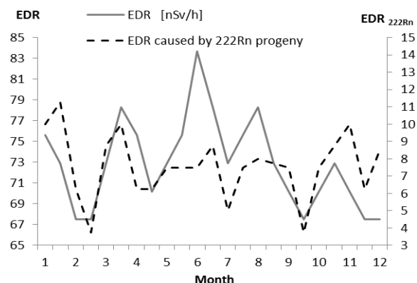
Figure 1. Variations of the total EDR and EDR caused by 222 Rn progeny in the underground car parking places
