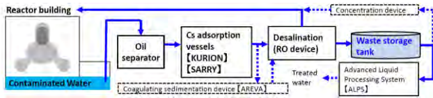
Figure 1. Decontamination system of SARRY, KURION and ALPS in Fukushima NPP-1.
