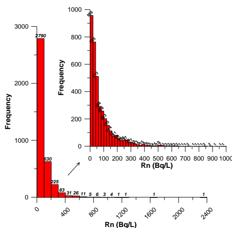
Figure 1. Histograms showing the distribution of radon concentrations of the 3,818 groundwater.
