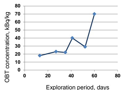
Figure 2. Changes of OBT concentration.
