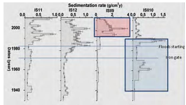
Figure 2. Isac lake mass sedimentation.
