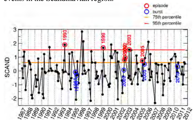
Figure 1. Monthly values of the SCAND index (black). In each year, six values, representing the cold months, are given. Red and blue circles annotate months when the cold episodes and bursts, respectively, are recorded. Orange and red lines are the 75 th and 95 th percentile thresholds for the SCAND distribution.
