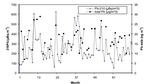
Figure 3. Concentrations for 210 Pb and the Pb total for years 2000–2005 in Helsinki, Finland.
