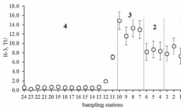
Figure 2. 3 H activity concentration in surface marine waters from west (Islandic coast) to east (South eastern Baltic) (1 – Baltic Sea, 2 – Kattegat, 3 – Skagerrak, 4 – North and Norwegian Seas)
