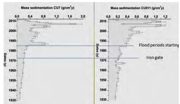
Figure 1. Cuibida lake mass sedimentation.
