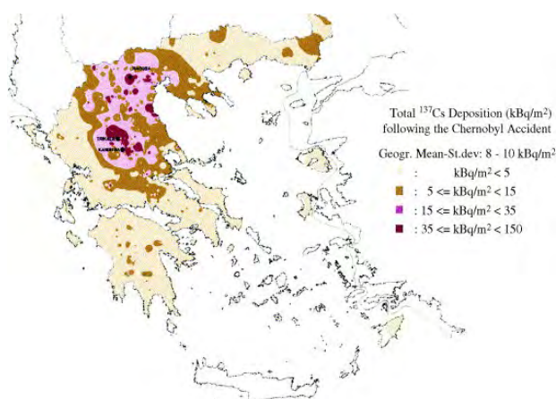
Figure 1. 137 Cs activity concentrations in surface soil samples in Greece during May-November 1986 (Petropoulos et al., 2001)
