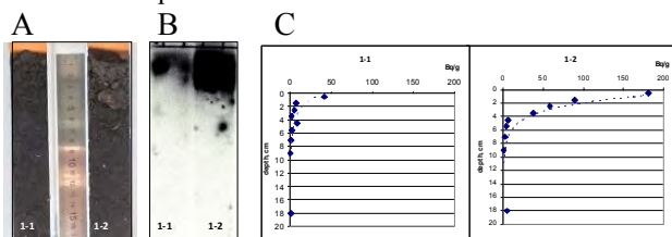
Figure 1. Distribution of ^{137}\text{Cs} in soil cores after growing oat: A – photography, B – digital autoradiography, C – \gamma -spectrometry
