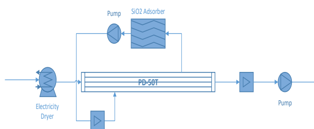
Figure 2. Structure of the continuous drying system
