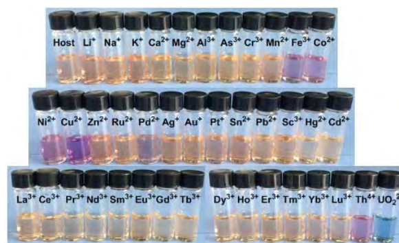
Figure 1. Image of the solutions of T-PADAP ( 10^{-5}\text{M} )/cation ( 10^{-5}\text{M} ) mixtures at a f_w of 40% taken under natural light.
