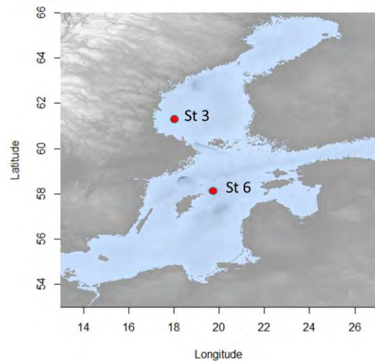
Figure 1. The two selected station in the Baltic Sea were radionuclide distribution have been studied in sediment cores.
