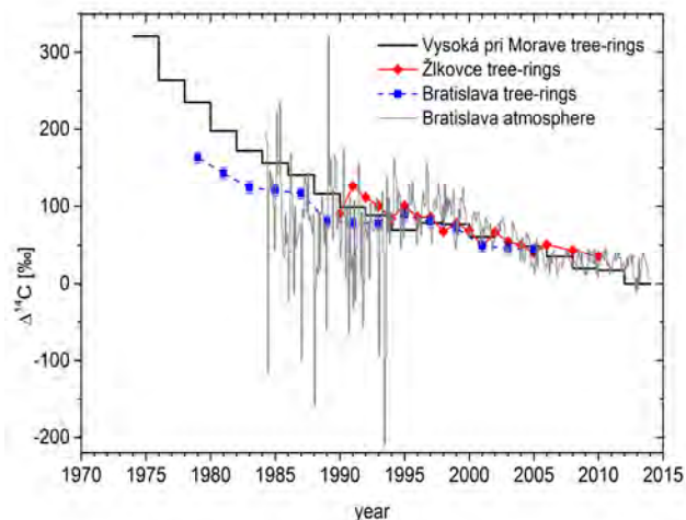
Figure 1. Radiocarbon concentration in annually growth rings from three sampling stations in Slovakia, and monthly atmospheric data from Bratislava. The Vysoká pri Morave data are shown as a histogram, because they represent two-year averages (Žilkovce and Bratislava results represent annual data).
