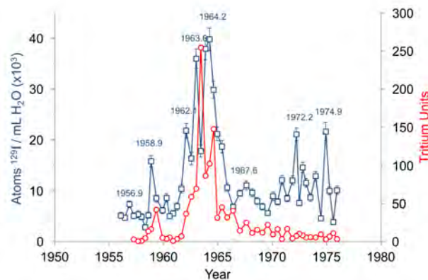
Figure 1. 129 I and tritium in the SE-dome ice core.
