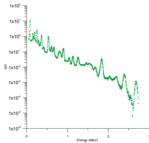
Figure 1: Total spectrum
