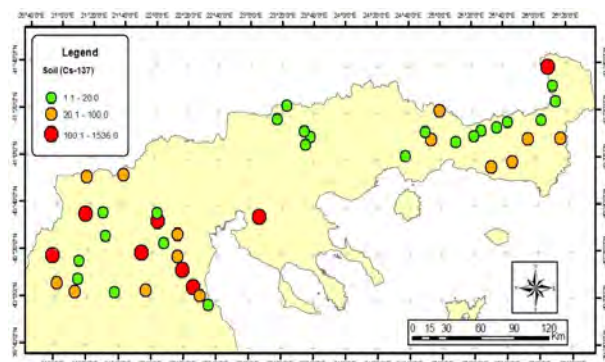
Figure 2. 137 Cs activity concentrations in surface soil samples in Northern Greece during July-September 2016 (present work - 46 samples analysed up to now)
