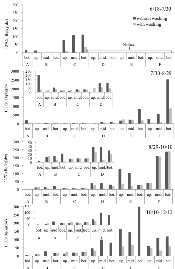
Fig. 2. Radiocesium concentrations in the aboveground parts of Komatsuna at each site
