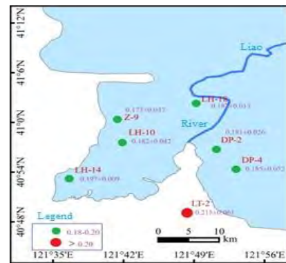
Figure 3. 240 Pu/ 239 Pu atom ratios of surface sediments in the Liao River estuary.
