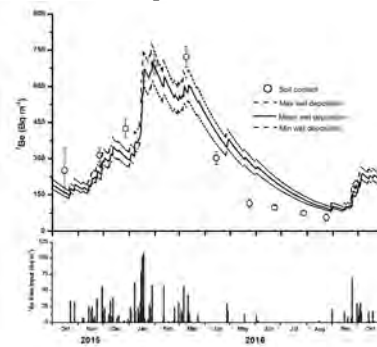
Figure 2. 7 Be wet deposition and 7 Be soil content (upper) and 7 Be input by rains (lower).
